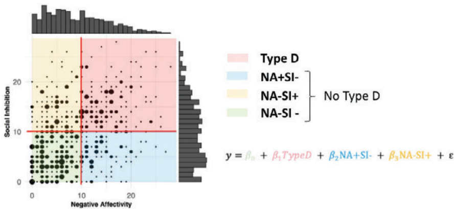
Figure 5: Scatterplot and histogram of the NA and SI sum scores (based on data from Chapter 7 ), indicating how the 4-group method transforms these scores into a nominal personality group variable using cutoff scores of 10 (two red lines). This nominal variable is typically dummy coded before including it in a regression equation.
