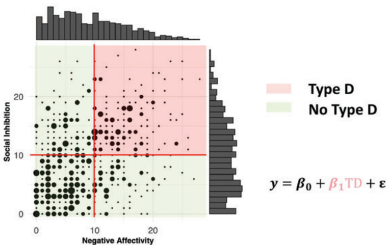
Figure 4: Scatterplot and histogram of the NA and SI sum scores (based on data from Chapter 7 ), indicating how the 2-group method transforms these scores into a dichotomous Type D variable using cutoff scores of 10 (two red lines) and how this resulting variable is typically included in a regression equation.
