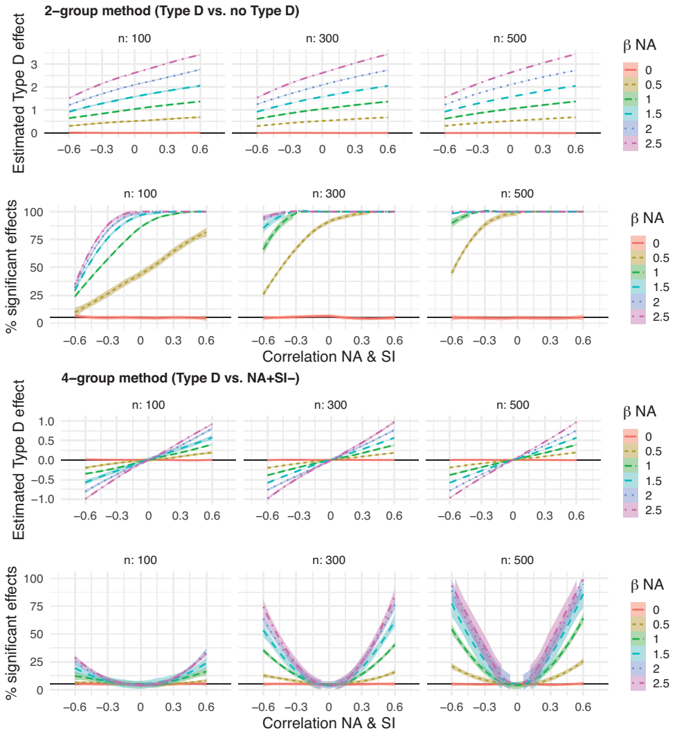
Figure 2: The estimated regression coefficients and proportion of significant effects of the 2-group method (upper two rows) and the 4-group method’s contrast between the Type D group and the group with high NA scores only (bottom two rows). The simulated datasets varied in sample size (columns), the correlation between NA and SI (x-axis) and the size of the true effect underlying the simulated data (i.e., NA main effect; separate lines). All other effects were fixed to zero.
