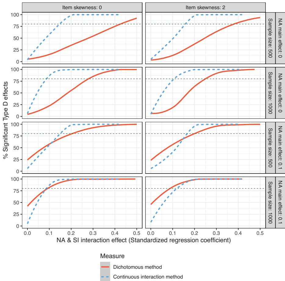
Figure C1: The percentage of significant Type D effects according to dichotomous method (red solid line) and continuous method (blue dashed line), varying over sample size, item skewness, the underlying NA main effect and NA*SI interaction effect. In all conditions, the size of the SI main effect was fixed to zero.
