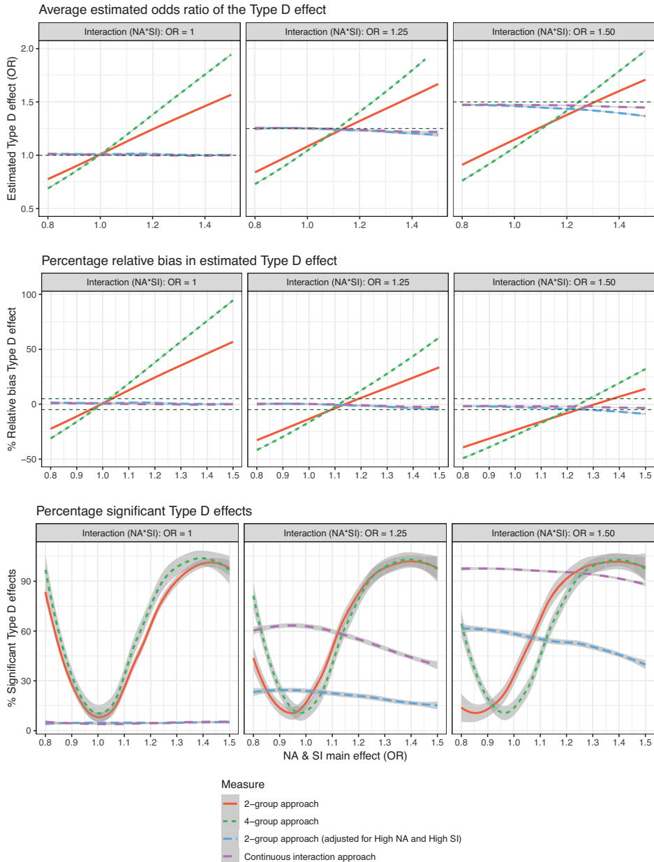
Figure 1: For each Type D operationalization and for varying levels of the Type D effect and the NA and SI main effects, the mean estimated odds ratio (upper), percentage relative bias (middle) and percentage significant results (lower) of the Type D effect.
